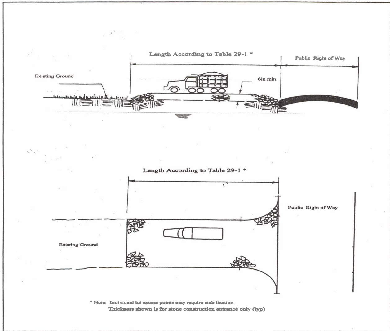
Figure 29-1: Stabilized Construction Access
