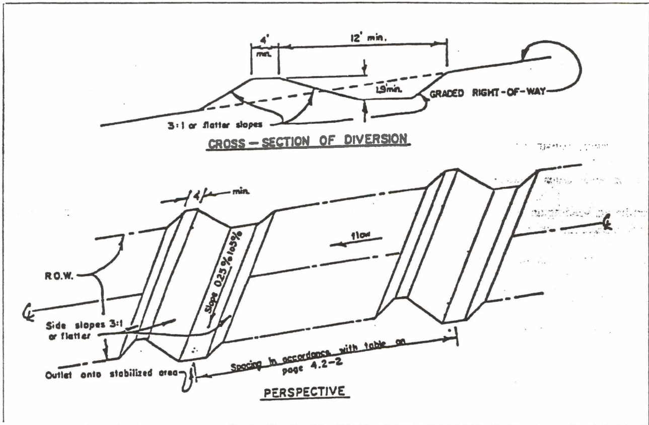
Figure 15-4 Detail of small diversions for roadbed right-of-way
