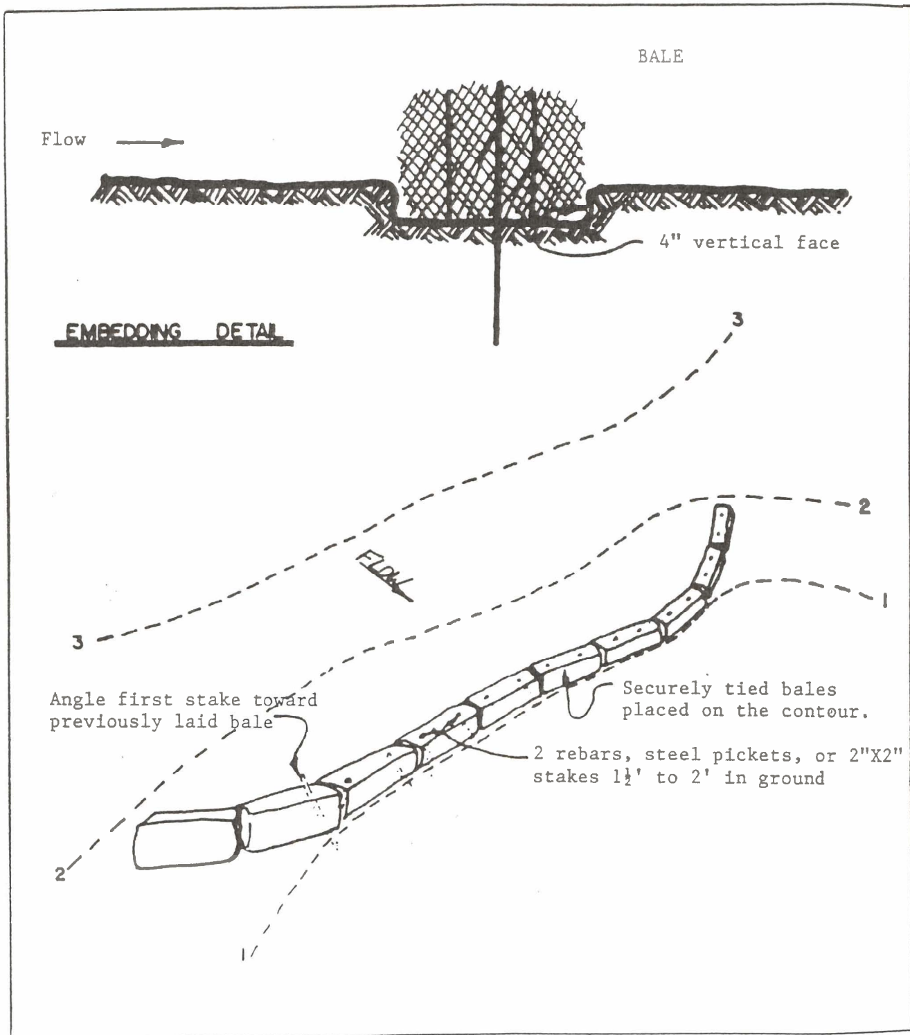
Figure 25-1 Placement and Anchoring Detail Bale Sediment Barriers
